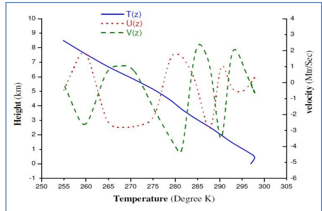
Fig. 9. Profile of U(z) , V(z) and T(z) on 15.08.2003
