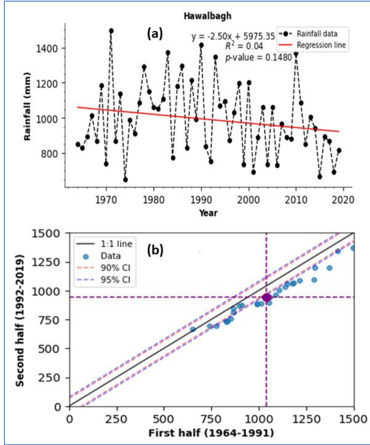
Figs. 3 (a&b). (a) Deterministic and (b) innovative trend plots of annual rainfall at Hawalbagh station (1964–2019).
