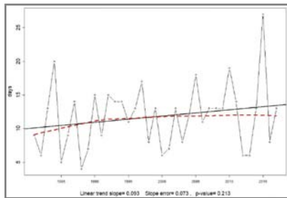
Annual count of days when PRCP &gt;10mm in PAP plain area
