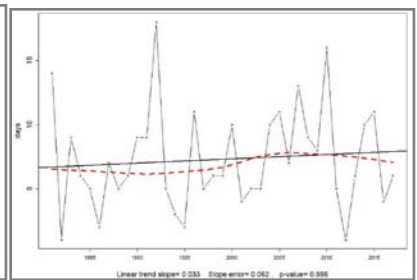
Annual count of days when PRCP &gt;30mm in PAP plain area
