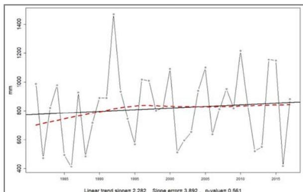
PRCPTOT in Aliyar sub-basin command area
