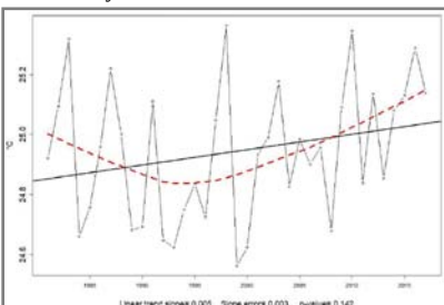
Annual mean daily maximum temperature of Aliyar sub-basin command area
