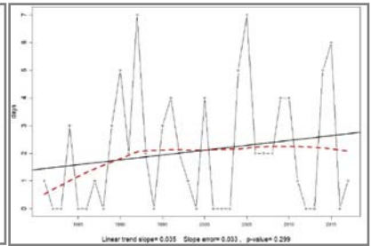
Fig. 4. Extremities on Rainfall (PRCP < 10mm, PRCP < 20mm, PRCP < 30mm) of PAP basin
