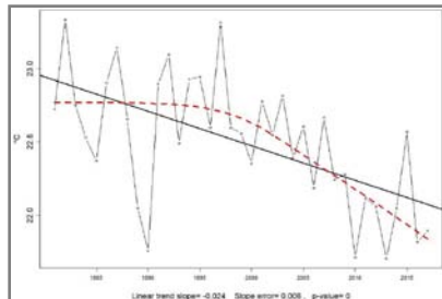
Annual mean daily minimum temperature PAP hilly area
