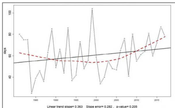
Consecutive dry days in Aliyar sub-basin command area
