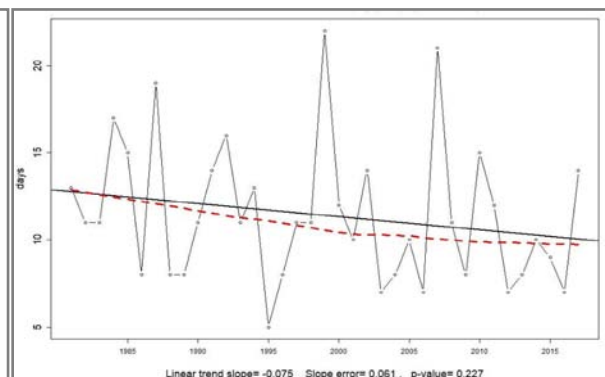
Consecutive wet days in Aliyar sub-basin command area
