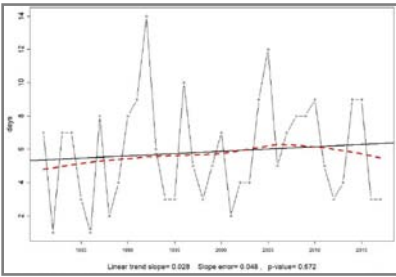
Fig. 4. Extremities on Rainfall (PRCP < 10mm, PRCP < 20mm, PRCP < 30mm) of PAP basin
