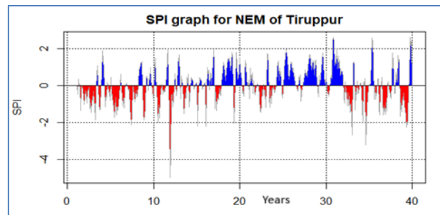
Fig. 3(b). SPI-3 pattern values for the district of Tiruppur from 1981 to 2019
