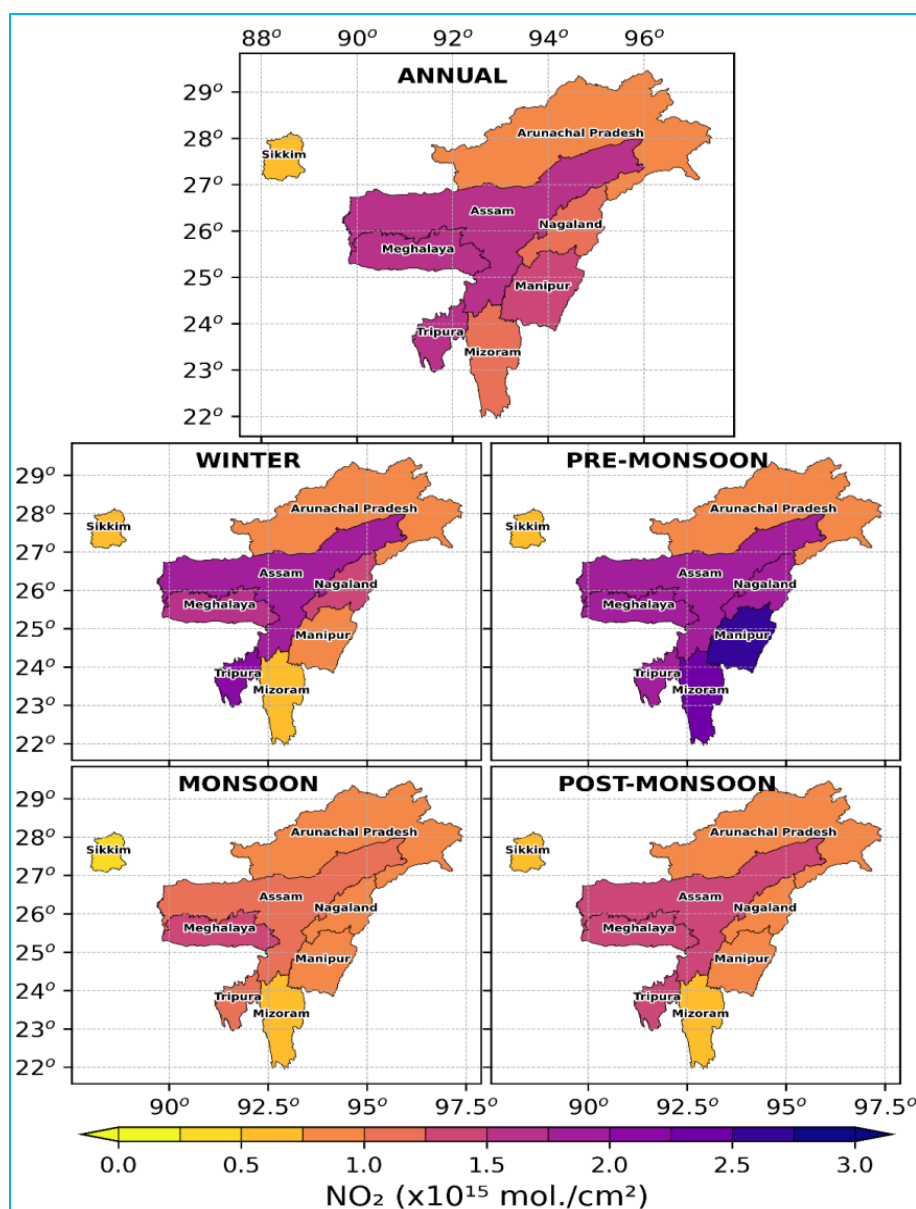
Fig. 3. Spatial distribution of mean TCN over the NERI (2005-2022)
