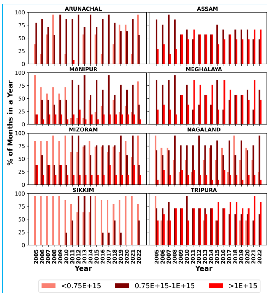
Fig. 10. Frequency analysis of \text{NO}_2 Concentrations in NERI
