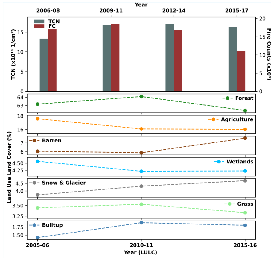
Fig. 8. Variations in TCN, fire counts and LULC types over the NER
