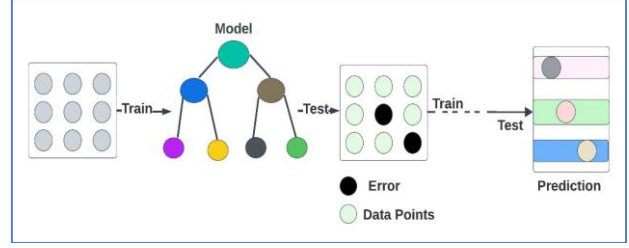
Fig. 5 Schematic of Light Gradient Boosting Machine (Light GBM) Regression
