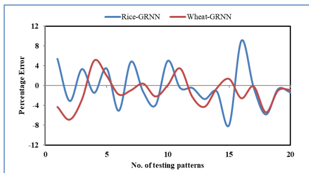
Fig. 9. Visual depiction of error percentage in GRNN testing data
