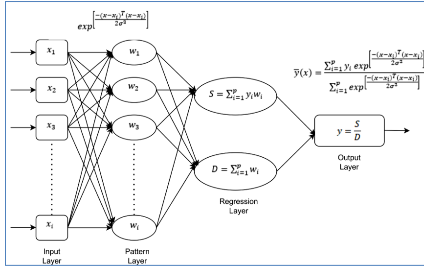
Fig. 4. Architecture of GRNN model
