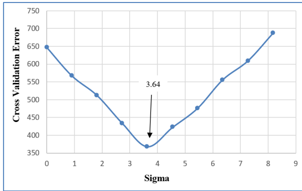
Fig. 5. Cross-validation curve for GRNN model
