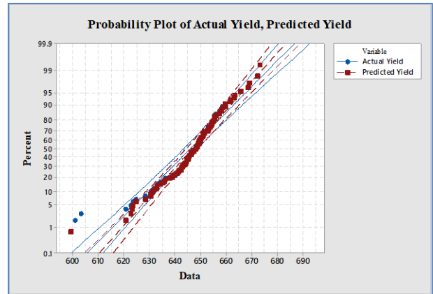
Fig. 6(a). Actual vs Estimated crop yield (rice) values in RSM model
