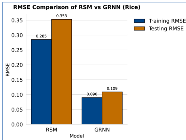
Fig. 11. RMSE comparison of GRNN and RSM models (rice yield)
