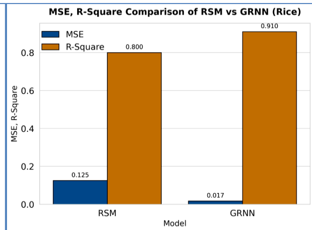
Fig.12. MSE &R-Square comparison of GRNN & RSM models (rice yield)
