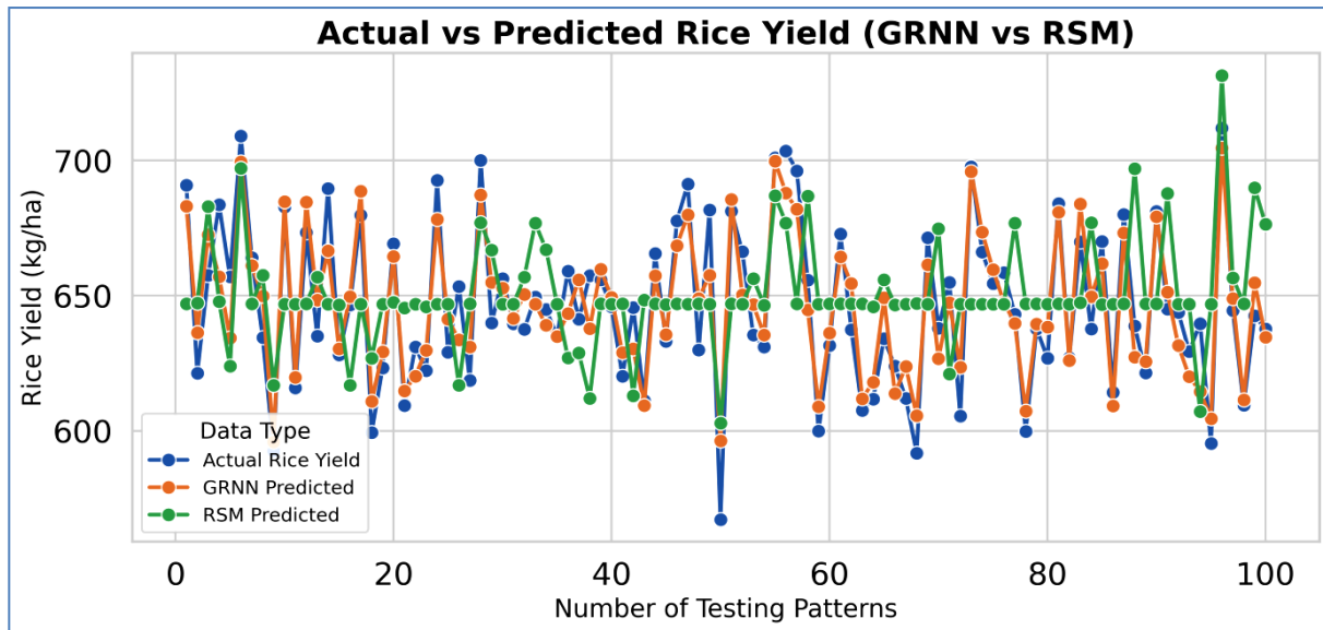
Fig. 15. Trends of GRNN - RSM along testing patterns (Rice yield)
