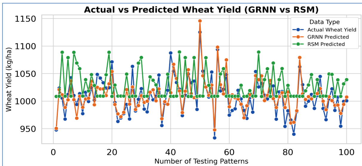
Fig. 16. Trends of GRNN - RSM along testing patterns (Wheat yield)
