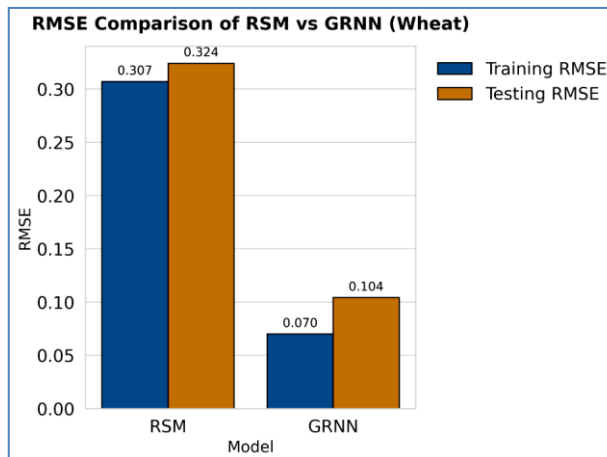
Fig. 13. RMSE comparison of GRNN and RSM models (wheat yield)
